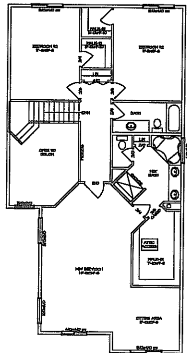
2ND FLOOR LAYOUT
