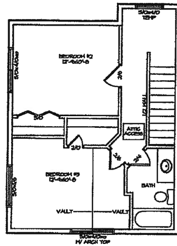
2ND FLOOR LAYOUT
