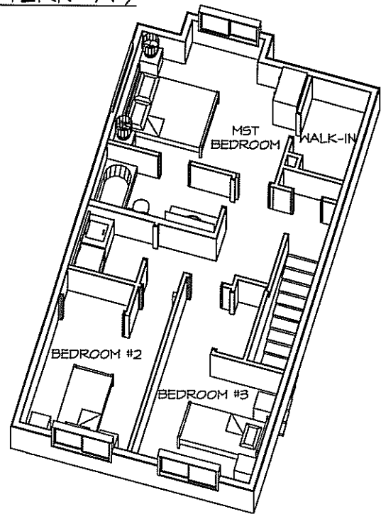
2ND FLOOR
